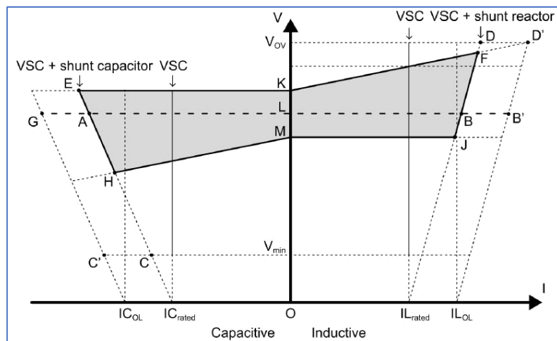
Figure-3: VI Curve of the STATCOM Station
