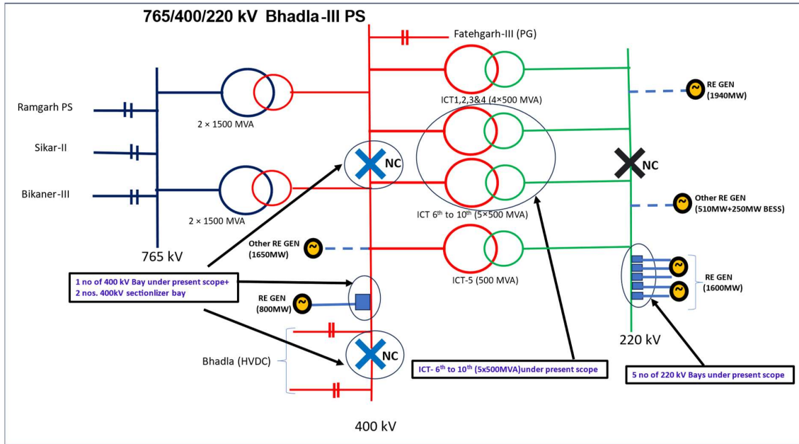
Fig-schematic of 765/400/220 kV Bhadla-III PS
