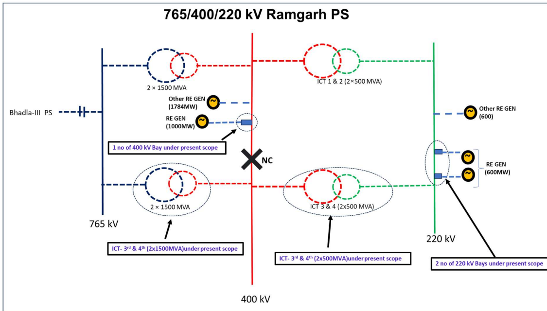
Fig-schematic of 765/400/220 kV Ramgarh PS
