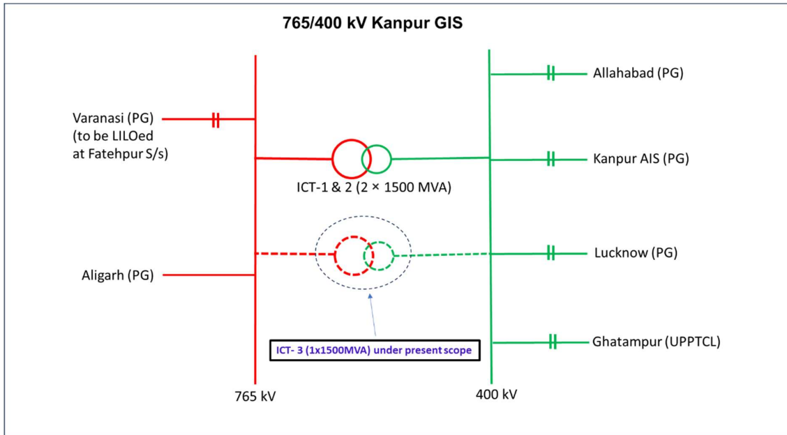
Fig-schematic of 765/400 kV Kanpur S/s
